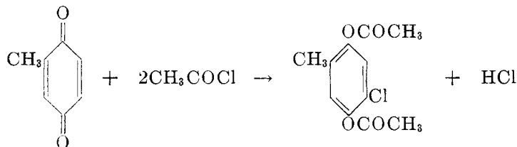
5-Chloro-2-methylhydroquinone diacetate
